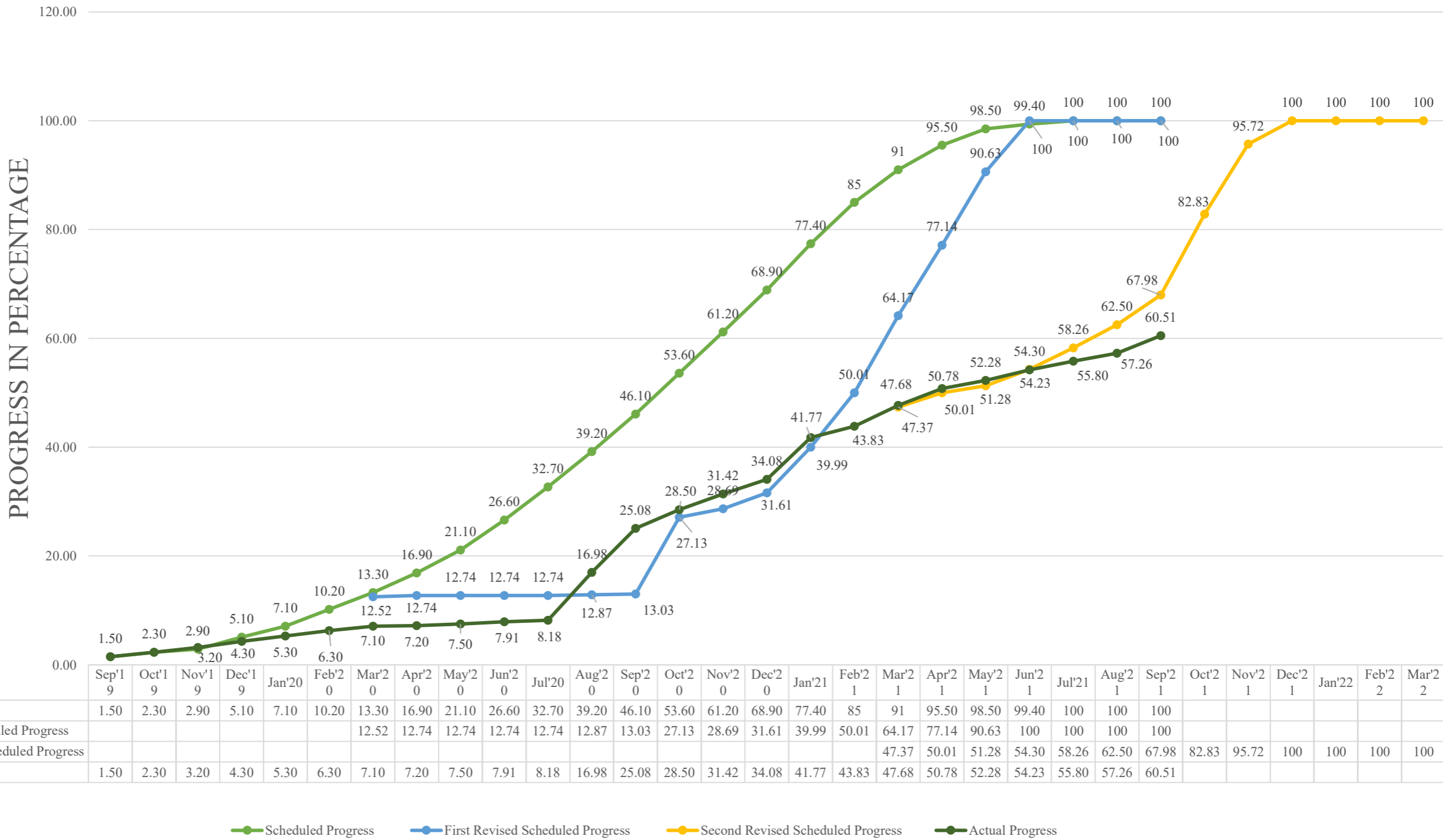
SCHEDULED Vs ACTUAL PROGRESS CHART OF PACKAGE - I
