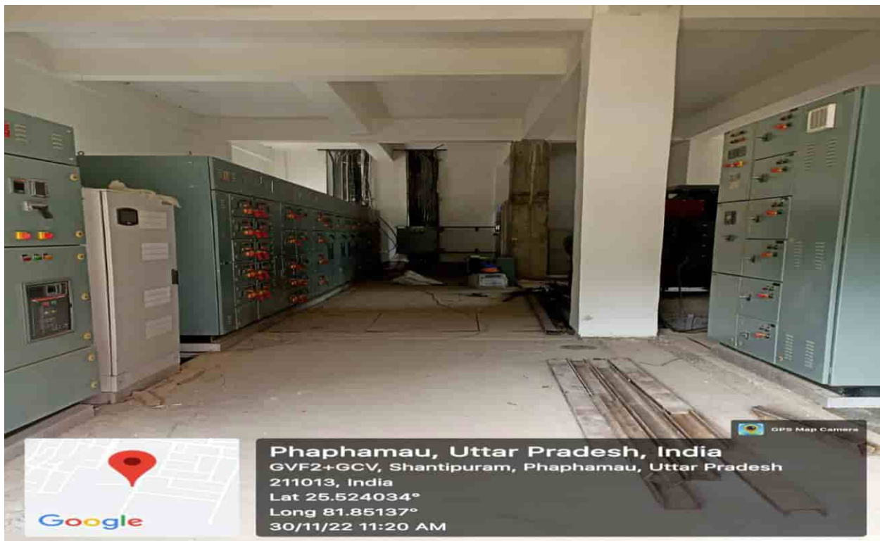
Process Building (STP) – PMCC panel erection work completed and cabling work under progress
