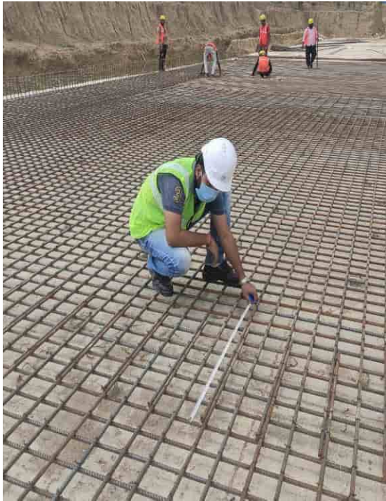
FCR –Reinforcement of bottom raft checked by Aecom Engineer
