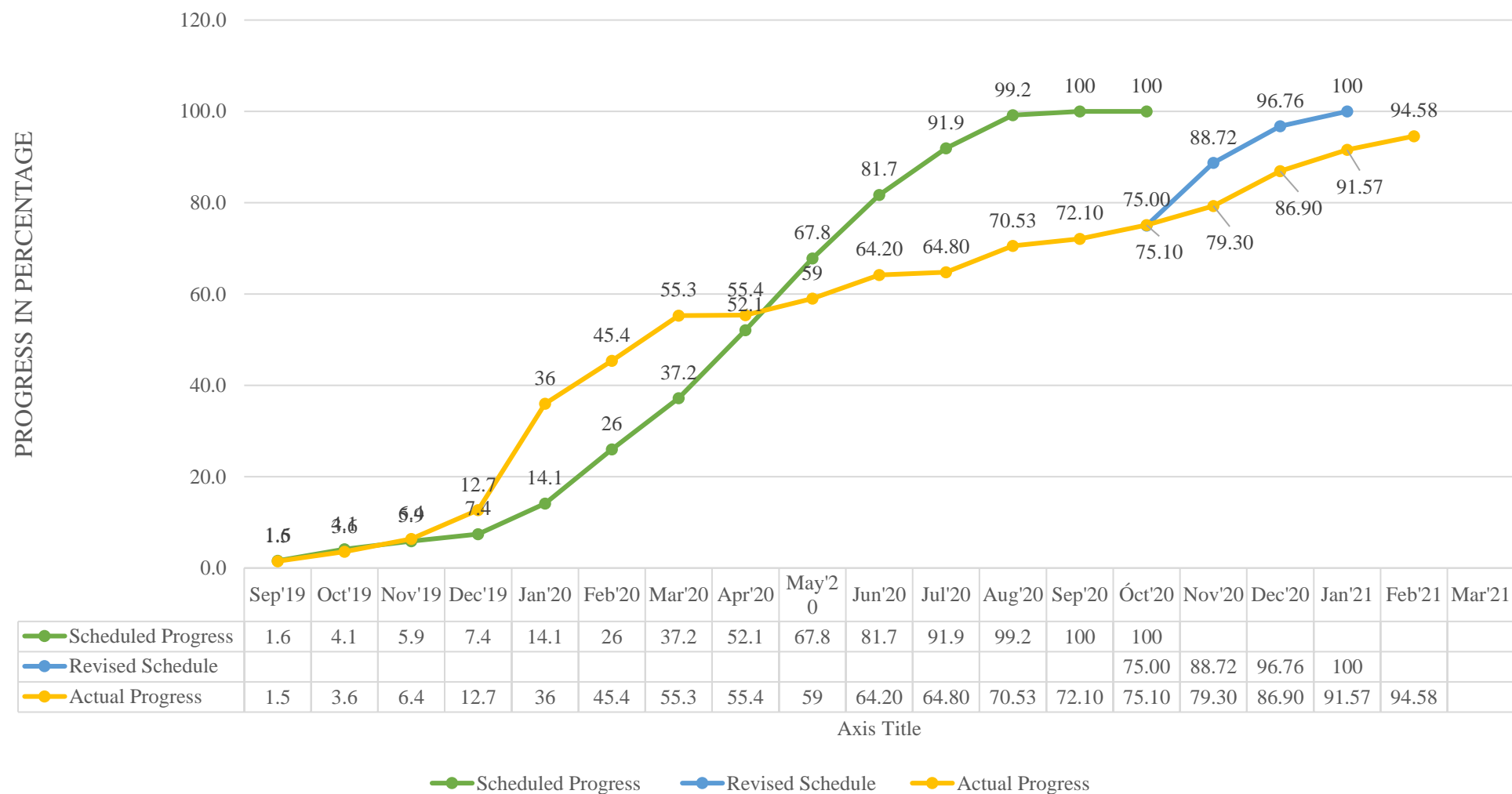
SCHEDULED Vs ACTUAL PROGRESS CHART OF PACKAGE - II
